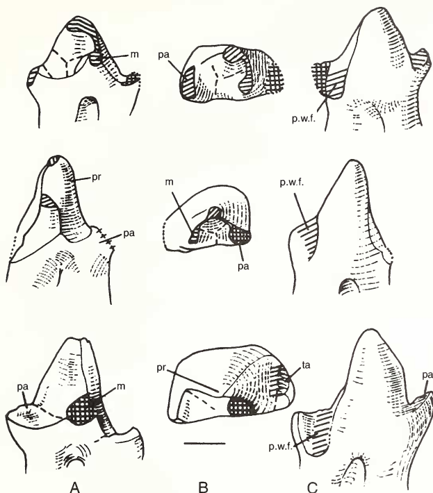
TEXT-FIG. 10. Lower molars of, from top to bottom: Araeodon , Paurodon , Archaeotricon brevimaxillus . A, lingual view; B, occlusal view; C, labial view. Scale bar represents 0.5 mm.
